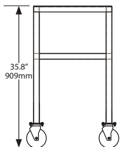
35.8" Oven Cart-Front
