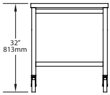
32" Oven Cart-Front
